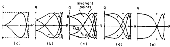
FIG. 1. Packet traces in the R - q plane. (Case \Delta n=3 , \Delta \mathbf{n}=2 .)
